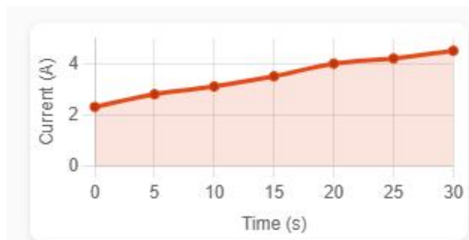
Fig. 8. Motor current (A) versus time (s).
