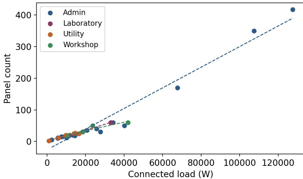
Fig. 6. Category-specific load-panel slopes fitted separately within each functional category, visualising the ANCOVA slope-homogeneity test ( F(3,27) = 2.52, p = .079 ).
