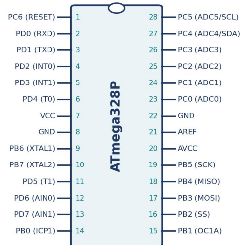
Fig. 2. ATmega328P microcontroller pin configuration.
